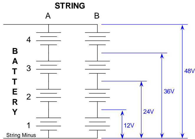
Figure 6: Battery String Naming Conventions
