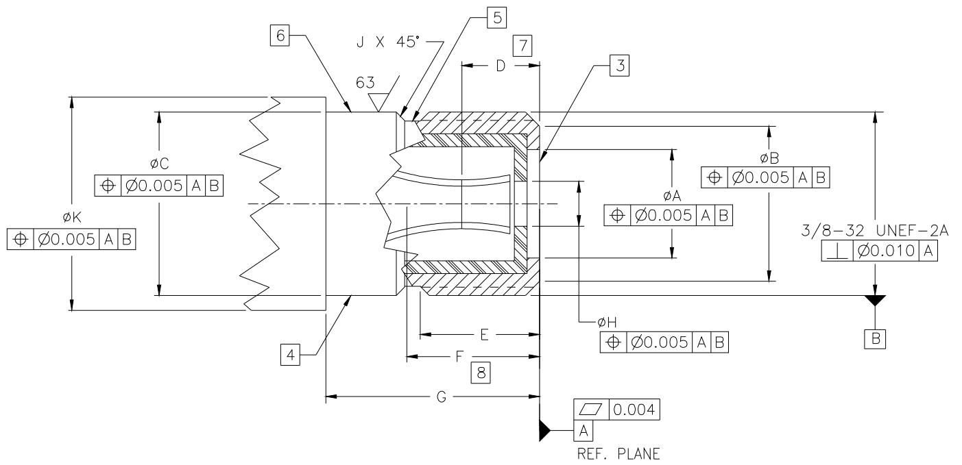
Figure 1 – Recommended Outdoor Female “F” Port
