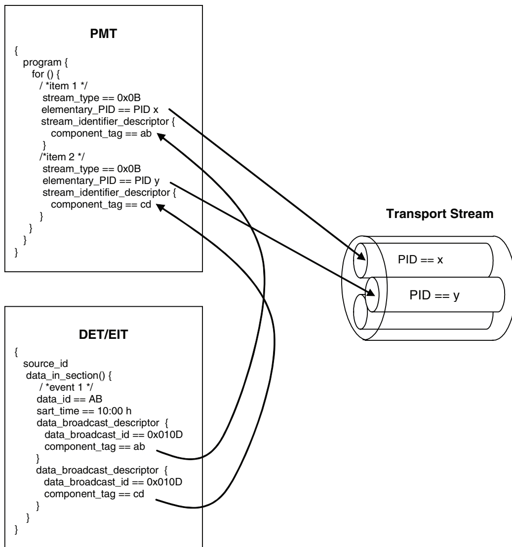
Figure 6.1 The Relationship of DET/EIT, PMT and ACAP data elementary stream through data broadcast descriptor. (Informative)
